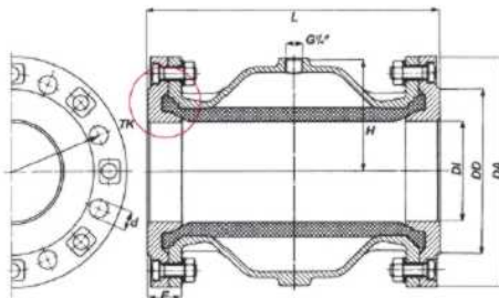
Standard Aluminium Standard aluminium
